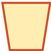
Figure 1.2: Isosceles trapezoid
